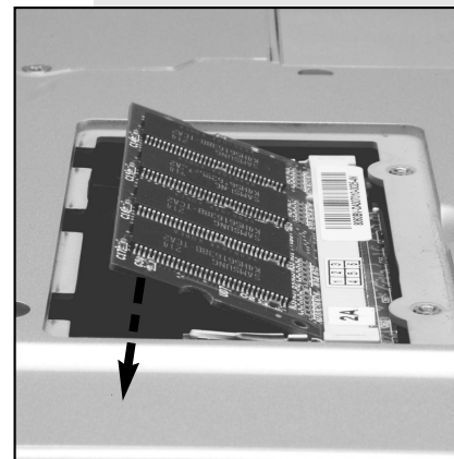
Figure 4.3: Replacing the Memory Card
