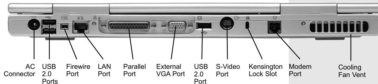
Figure 1.3: Rear View of the WinBook Notebook
