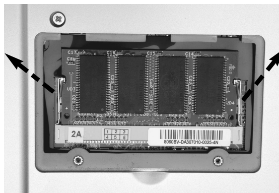
Figure 4.2: Replacing or installing RAM
