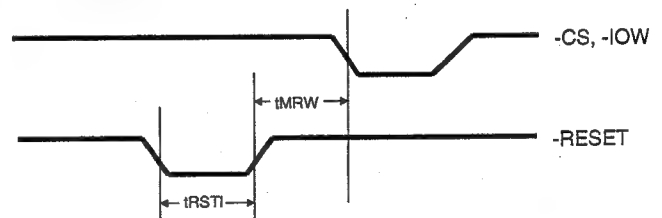
Fig. 4-24: HDD Program I/O Read Timing
