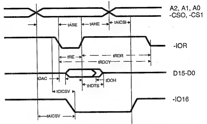
Fig. 4-23: HDD Program I/O Read Timing
