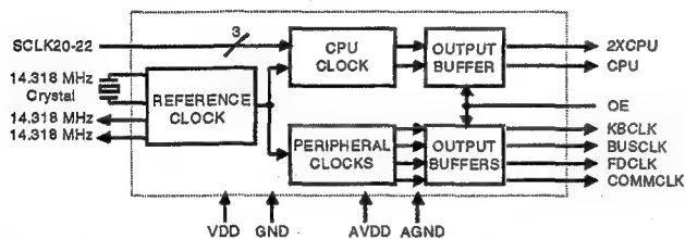
Fig. 4-2: Block Diagram
