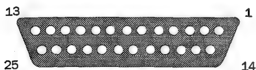
Fig. 4-13: Parallel Port
