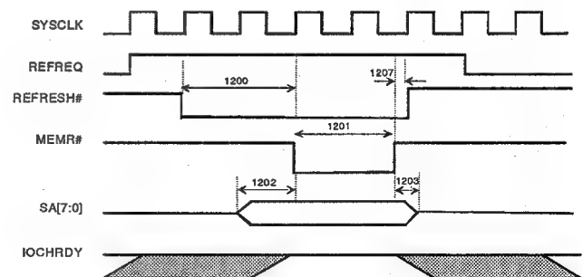
Fig. 4-5: AT Bus Refresh Timing
