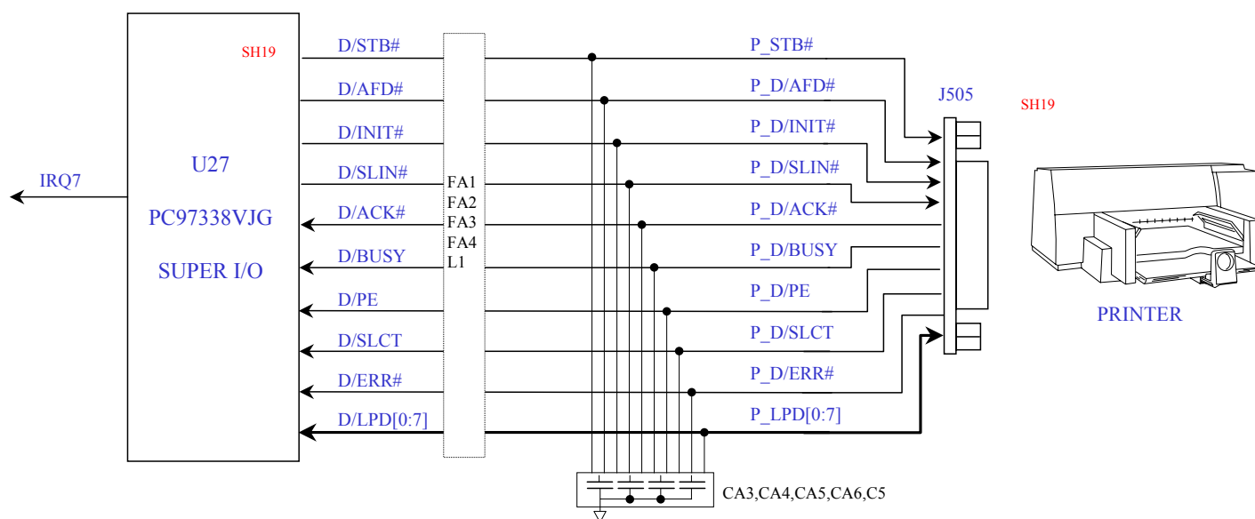
PIN DEFINITION OF PIO PORT
